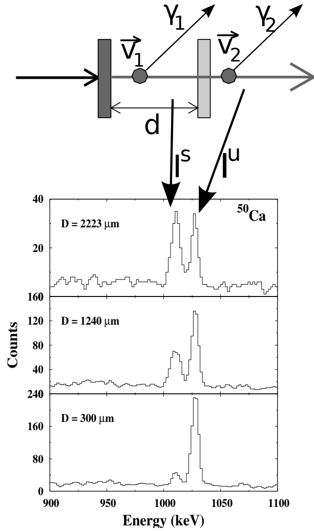
Figure 3.1: Schematic illustration of lifetime measurements using the RDDS method. v_1 and v_2 correspond to recoils velocities before and after the degrader placed at a distance d after the target. The corresponding peaks intensities are denoted I^s and I^u . The evolution of the peak intensity of the shifted ( I^s ) and unshifted ( I^u ) components as a function of the target-degrader distance is given in the case of ^{50}\text{Ca} [65].
