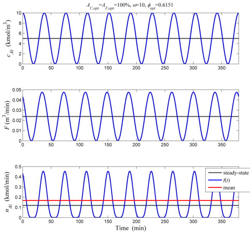
Figure 4.12 The modulated inlet concentration of the reactant (top), and flow-rate (middle), for simultaneous modulation of these two inputs with dimensionless forcing frequency \omega=10 , optimal forcing amplitudes A_C=A_F=100\% , and optimal phase difference \phi_{opt}=0.6151 , and the inlet molar flow-rate of the reactant (bottom)
