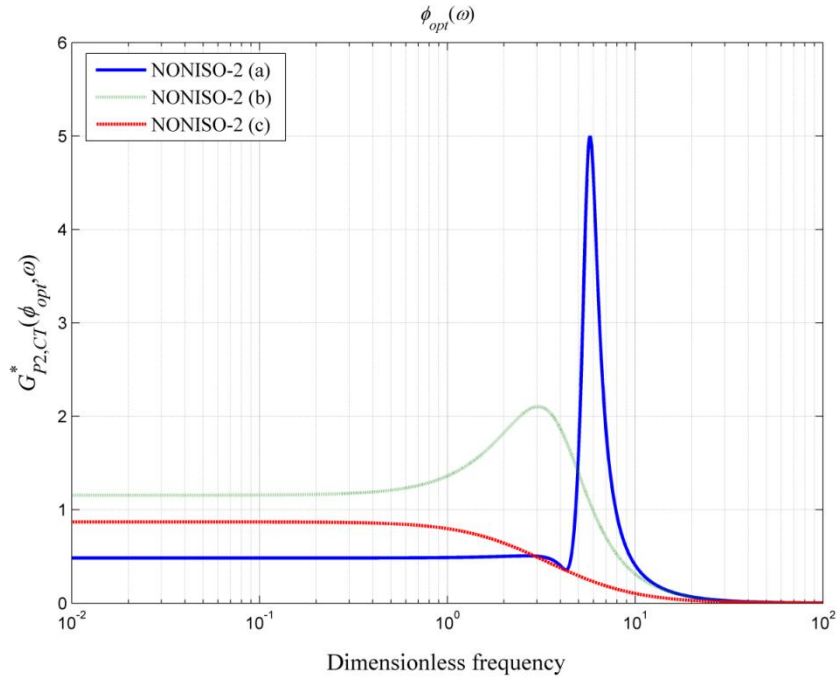
Figure 4.18 The cross ASO terms corresponding to the optimal phase differences, ( G_{P2,CT}^*(\phi_{opt},\omega) ) as functions of the dimensionless forcing frequency, for Numerical examples NONISO-2(a), NONISO-2(b) and NONISO-2(c)
