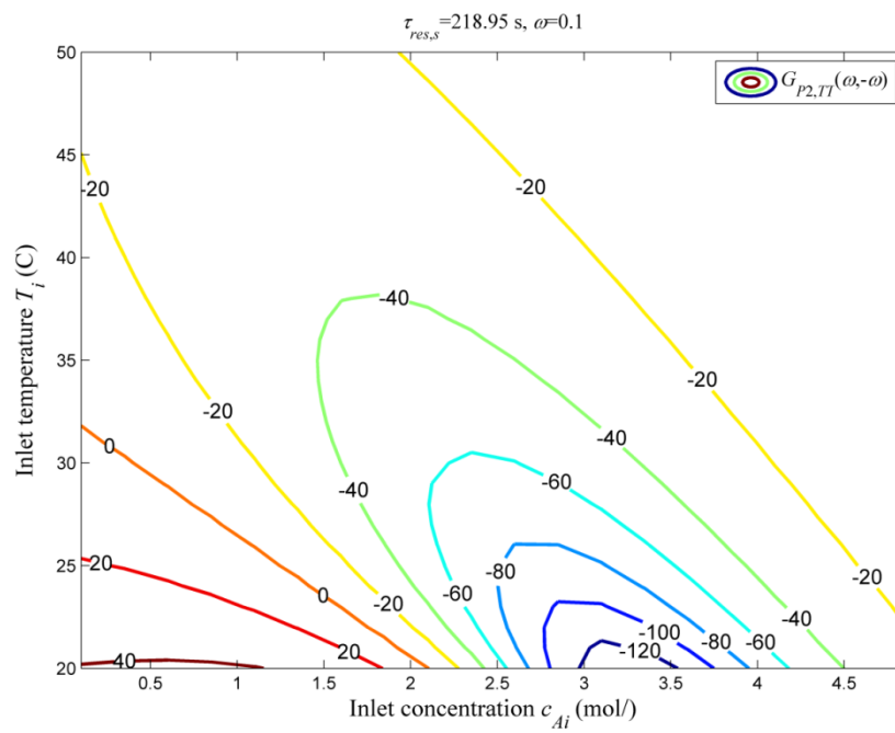
Figure C2 The ASO FRF G_{P2,TT}(\omega, -\omega) as a function of the inlet temperature and inlet concentration of the reactant, for constant residence time \tau_{res,s}=218.95 s and dimensionless forcing frequency \omega=0.1
