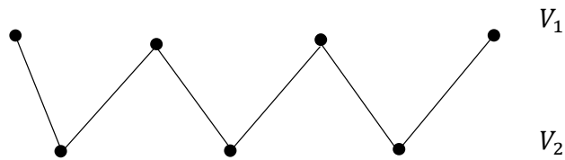
Figure 1.5.6 A diagram of a bipartite graph
