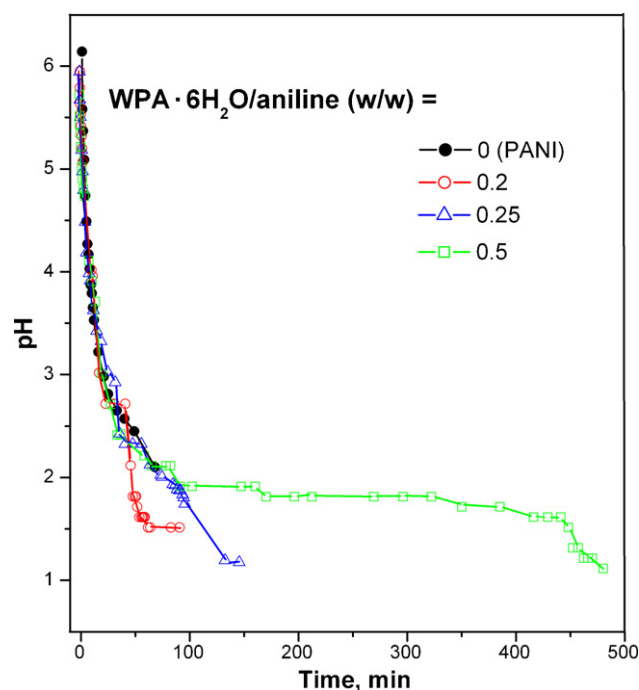
Fig. 2. Acidity profiles of aniline (0.1 M) oxidation with APS (0.125 M) in water at various initial WPA-6H 2 O/aniline weight ratios.
