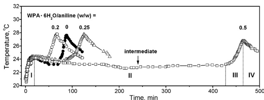
Fig. 1. Temperature changes during the oxidation of aniline (0.1 M) with APS (0.125 M) in water at various initial WPA-6H 2 O/aniline weight ratios: (○) 0.2, (△) 0.25 and (□) 0.5, and without added WPA (●). Phases I–IV correspond to the course of aniline polymerization in the presence of WPA, for the initial WPA-6H 2 O/aniline weight ratio = 0.5.
