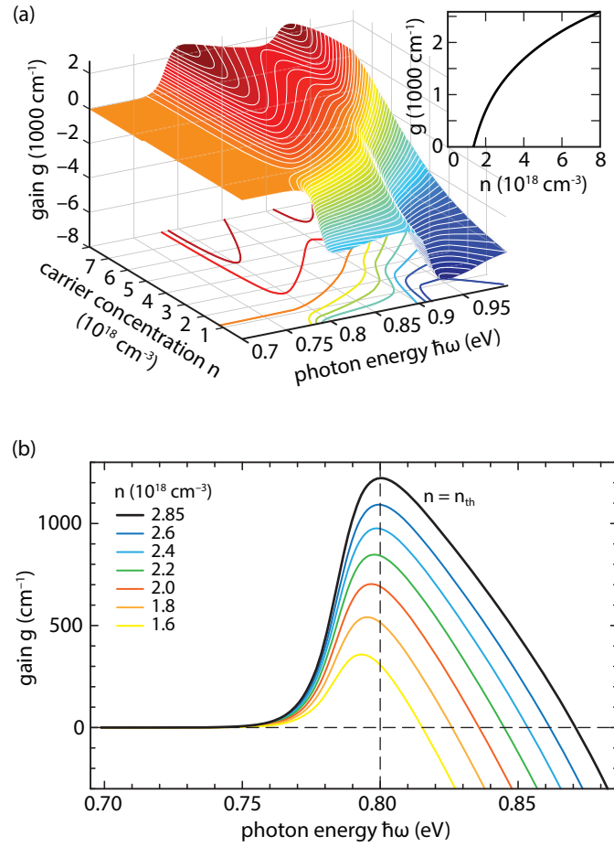
Figure 3.2: (a) Material gain spectrum for In_{0.75}Ga_{0.25}As_{0.87}P_{0.13} 1.05% compressive well with In_{0.46}Ga_{0.39}Al_{0.15}As 0.5% tensile barrier versus photon energy ( \hbar\omega ) and carrier concentration ( n ). Inset: Gain versus carrier concentration at \hbar\omega_0 = 0.8 eV. (b) Gain profile versus photon energy for different levels of carrier concentration [114].
