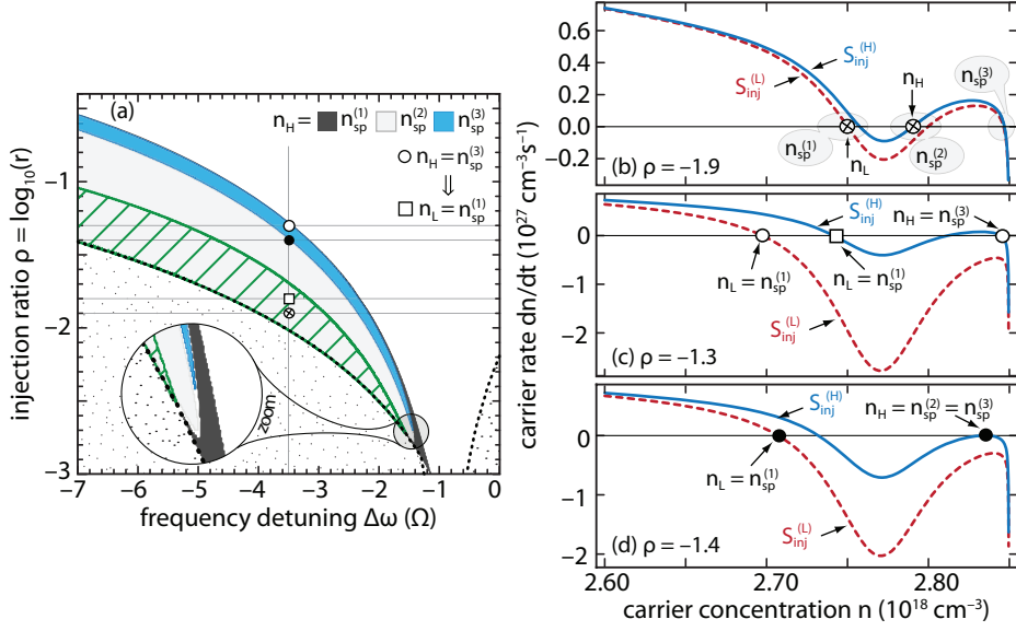
Figure 4.2: (a) Partition of the H -region, with respect to the type of the stationary point n_H . The n_L point from the H -region always maps into n_{sp}^{(1)} point, while n_H may map into n_{sp}^{(1)} (thin black area), n_{sp}^{(2)} (grey area), or n_{sp}^{(3)} (blue area). The hatched region represents an area in which n_L = n_{sp}^{(1)} coexist with n_H = n_{sp}^{(3)} , sharing the same injection power. (b) dn/dt-n plot and mapping of n_L and n_H into stationary points for \Delta\omega = -3.5\Omega and \rho = -1.9 . Same for (c) \rho = -1.3 and (d) \rho = -1.4 . In (c) n_L for \rho = -1.8 (rectangular dot) coexists with n_H for \rho = -1.3 (circular dot), sharing the same injection power. [115]
