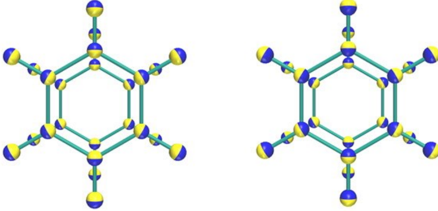
Figure 9.1.3. Schematic representation of a symmetric \vec{Q}_e (left) and anti-symmetric distortion \vec{Q}_o (right) of the benzene dimer. The size of vibrational motion on a nucleus is represented as sphere with the radius depending on the magnitude of the motion. The different colours indicate the direction of the motion.
