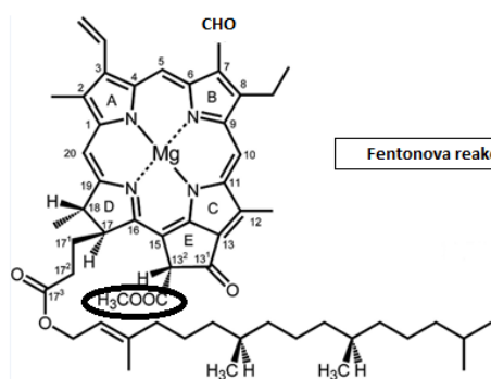
Pheob
