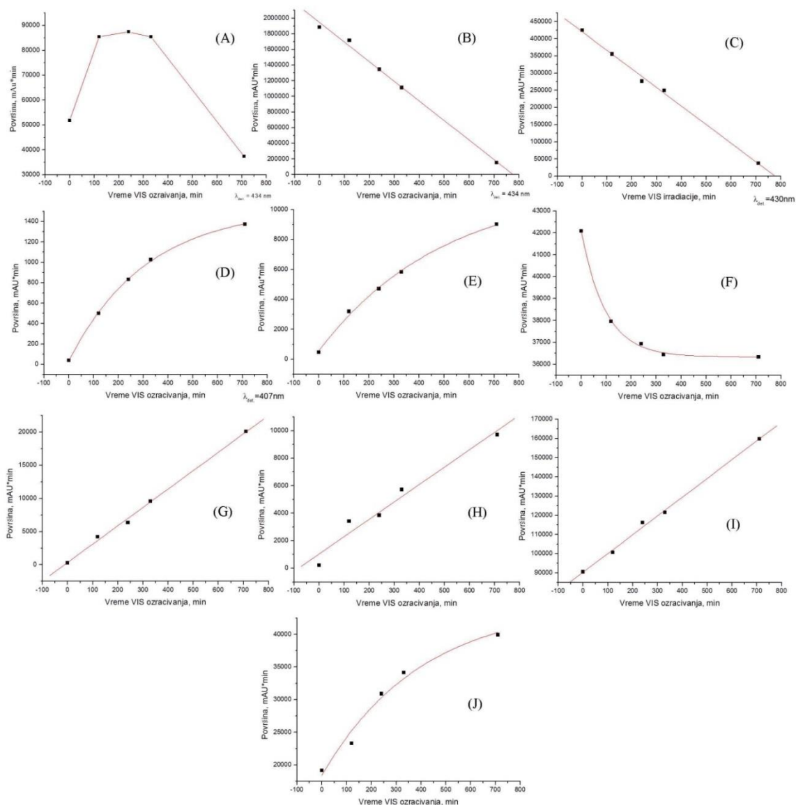
Slika 48. Dinamika promene površine pikova sa hromatograma prikazanog na Sl.47 (A) t_{ret.}=2.03 OH-Chla, (B) t_{ret.}=2.28 min, Chla, (C) t_{ret.}=2.45 min, Chla', (D) t_{ret.}=2.87 min, nepoznata komponenta, (E) t_{ret.}=2.96 min, OH-lakton Pheoa, (F) t_{ret.}=3.36 min, Pheob, (G) t_{ret.}=3.82 min, OH-Pheoa, (H) t_{ret.}=4.02 min, OH-Pheoa', (I) t_{ret.}=4.60 min, Pheoa, (J) t_{ret.}=5.06 min, Pheoa'.
