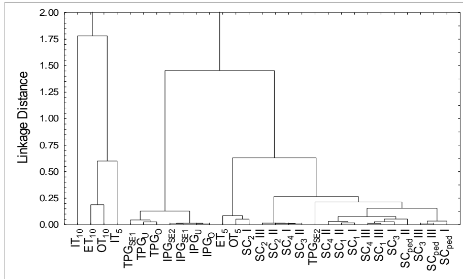
Figure 4.3.1. Dendrogram resulting from the Ward's method of hierarchical cluster analysis of SIRM values in the S. girensobnii moss. The exposure heights: I – 4 m; II – 8 m, and III – 16 m, in five street canyons ( SC_{1-4} , SC_{ped} ); the exposure positions in the tunnel: inside – IT, entrance – ET, outside – OT; exposure duration – five and ten weeks; exposure positions in different types of parking garages: T – tollgate and I – interior ( PG_{SE} – semi-enclosed; PG_O – open; PG_U – underground).
