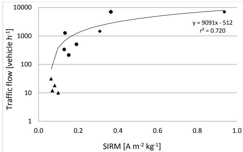
Figure 4.3.2. Correlation ( p < 0.05 ) shown on logarithmic scale between traffic flow (vehicles per hour) and the SIRM ( \times 10^{-5} \text{ A m}^{-2} \text{ kg}^{-1} ) measured in the S. girgensohnii moss, observed at \approx 4 \text{ m} in the street canyons (●) and a city tunnel (◆), and at \approx 2.5 \text{ m} in the parking garages (▲); n = 8 per studied position.
