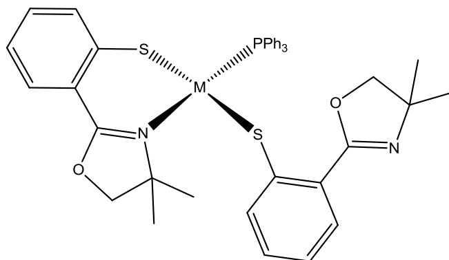
Slika 21. Struktura kompleksa [Pt(\eta^2S\text{-Phoz})(\eta^1S\text{-Phoz})(PPh_3)] , K6 .
