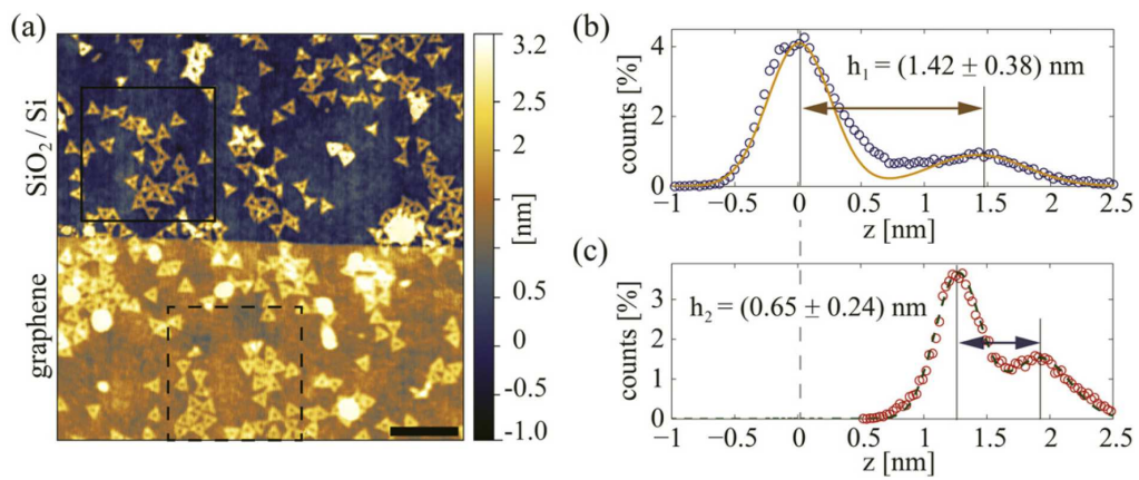
Figure 6.9.: (a)TAFM topography of a step edge of graphene covering a substrate with DNA origami nanostructures. Scale bar is 500 nm. (b) and (c) histograms (circles) and Gaussian fits (solid and dashed lines) of the selected areas in (a), corresponding to the bare and graphene encapsulated nanostructures. h_1 and h_2 stand for the height of the bare and graphene encapsulated structures, and are estimated as a peak-to-peak distance within the corresponding histograms. Figure taken from [423]
