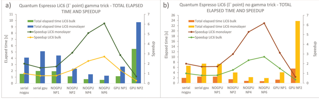
Figure 5.32.: Elapsed time and speedup for bulk and monolayer LiC 6 using Quantum Espresso, a) with gamma trick b) without gamma trick usage
