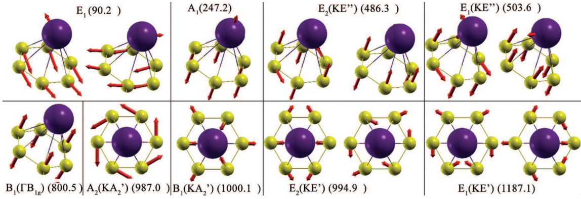
Figure 5.5.: Vibrational frequencies (in wave numbers) and normal coordinates for the monolayer \text{CaC}_6\text{-mono} . The modes of graphene with a similar displacement pattern are denoted in parentheses.
