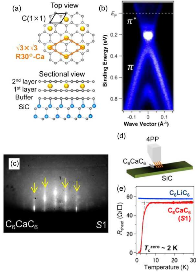
Figure 2.12.: Superconductivity of the Ca-intercalated bilayer graphene. (a) Schematic view of the crystal structure of C_6CaC_6 on SiC. (b) Band dispersions at the K point of pristine bilayer graphene obtained by ARPES. (c) RHEED pattern showing (\sqrt{3} \times \sqrt{3})E30^\circ spots and streaks. (d) Schematic diagram of the four-point-probe measurement setup. (e) Comparison of temperature dependence of sheet resistance R_{sheet} between C_6LiC_6 and C_6CaC_6 . Image from Ichinokura S et al [179]
