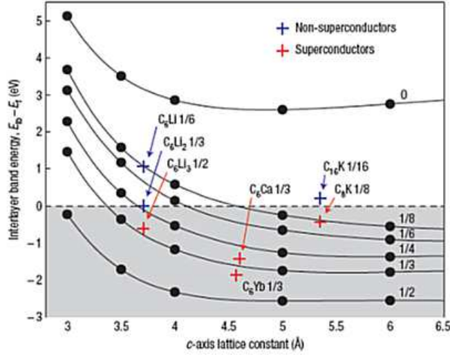
Figure 5.1.: The dependence of the interlayer band energy (at the \Gamma point) of the empty graphite system with changing c -axis spacing for different electron dopings. The interlayer band is occupied in the systems that fall into the shaded area. Figure taken from [254].
