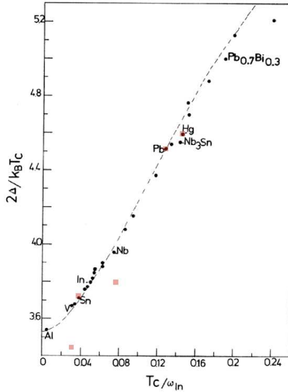
Figure 2.6.: The gap ratio 2\Delta_0/(k_B T_c) as a function of T_c = \omega_{In} . The black circles indicate theoretical calculations, with some of the elements and a couple of binary alloys indicated. The unmarked circles refer various binary alloys. Note the excellent agreement of theory with experiment in the case of Sn, Pb and Hg. Figure taken from [136].
