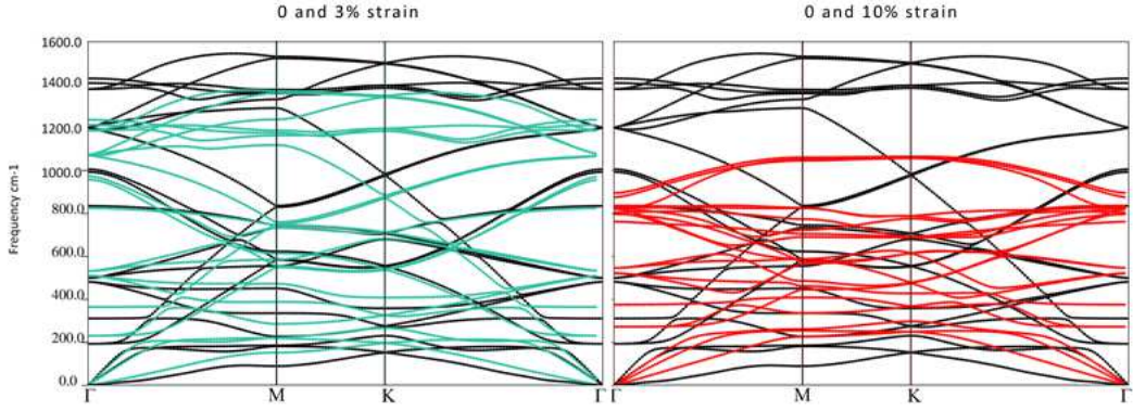
Figure 5.12.: Phonon dispersion for the \text{LiC}_6\text{-mono} , black lines as for the non-strained the \text{LiC}_6\text{-mono} and green and red for the 3% and 10% tensile biaxial strain, respectively.
