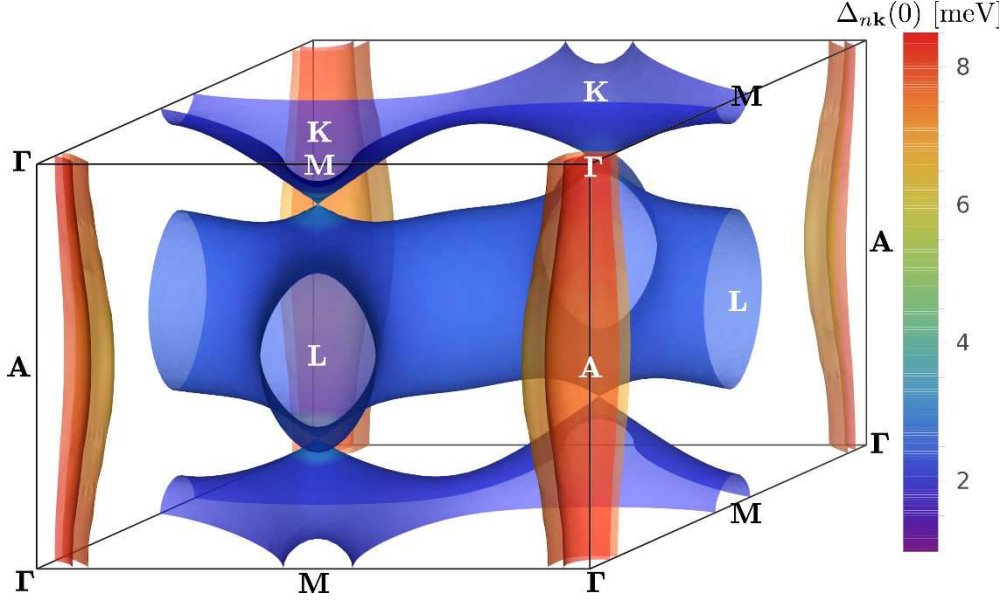
Figure 1.20.: The superconducting energy gap of MgB 2 , calculated at T \sim 10 K, mapped on the Fermi surface. The Fermi surface consists of two \sigma sheets along the \Gamma - \Gamma lines, and two \pi sheets along the K-M and the H-L lines (figure from [98], figure generated by [427])
