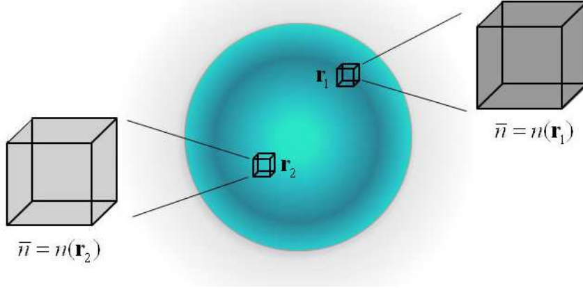
Figure 3.2.: In LDA at each point r , we can replace the exact xc energy density with that of a uniform homogeneous (hom) electron gas who has same density n(r)
