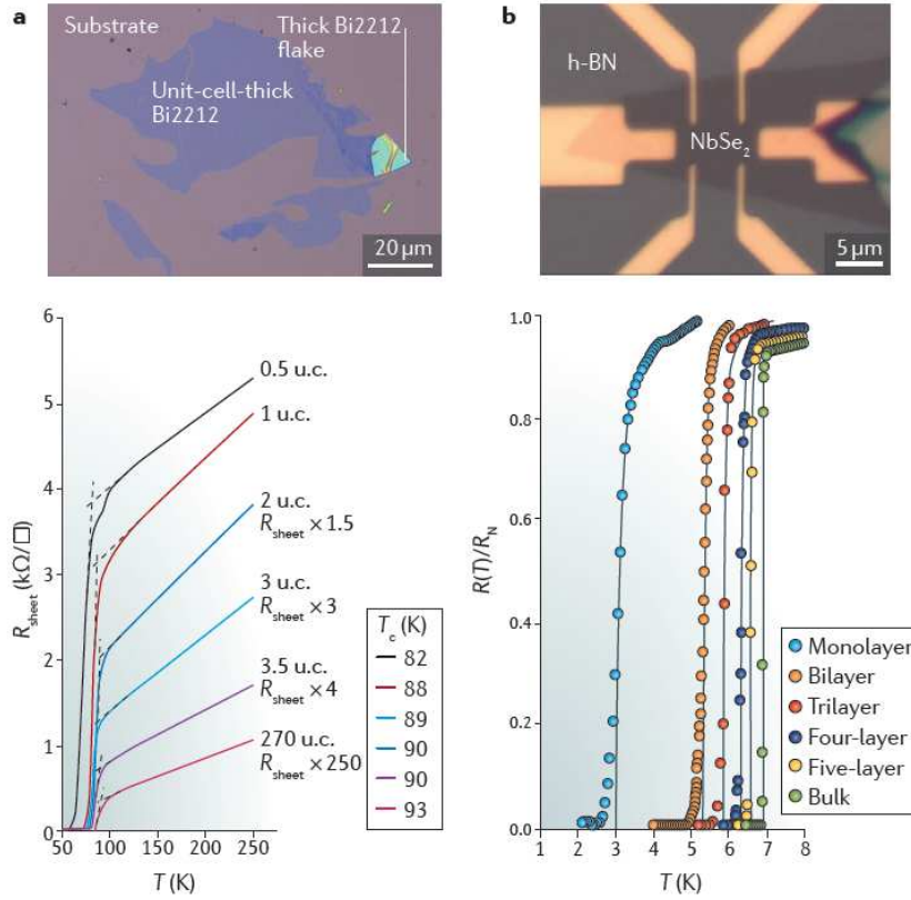
Figure 2.9.: Atommally thin superconductors based on exfoliated 2D crystals. a) Optical microscope image showing \text{Bi}_2\text{Sr}_2\text{CaCu}_2\text{O}_{8+x} (Bi2212) flakes (top). Temperature ( T )-dependent sheet resistance, R_{\text{sheet}} , for Bi2212 samples with various thicknesses, ranging from 270 unit cells to half a unit cell (u.c.; bottom). b) Optical image of a bilayer \text{NbSe}_2 device capped by a thin hexagonal boron nitride (h-BN) layer for environmental protection (top). Resistive superconducting transition of \text{NbSe}_2 samples with different thicknesses, ranging from atomic thickness to bulk (bottom). R_N , onset resistance; T_c , superconducting transition temperature. Figure from the [194]
