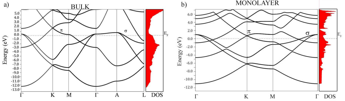
Figure 5.22.: The Electronic band structure and the total density of states of the \text{MgB}_2 bulk and the monolayer.
